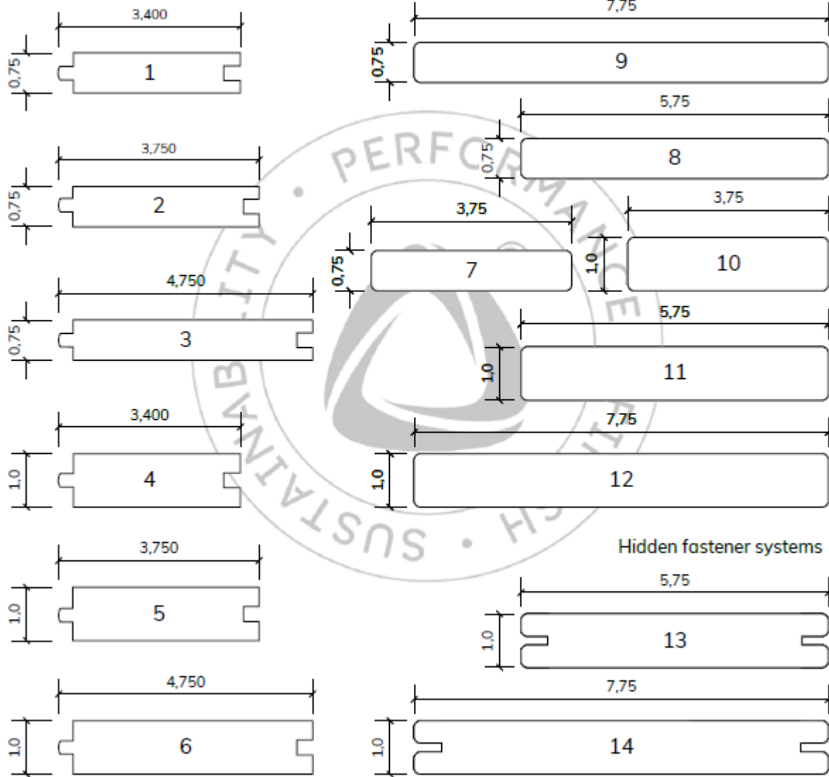
FIGURE 1—ACCOYA LUMBER PROFILES
