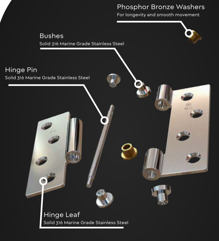
HQ4 Hinge
